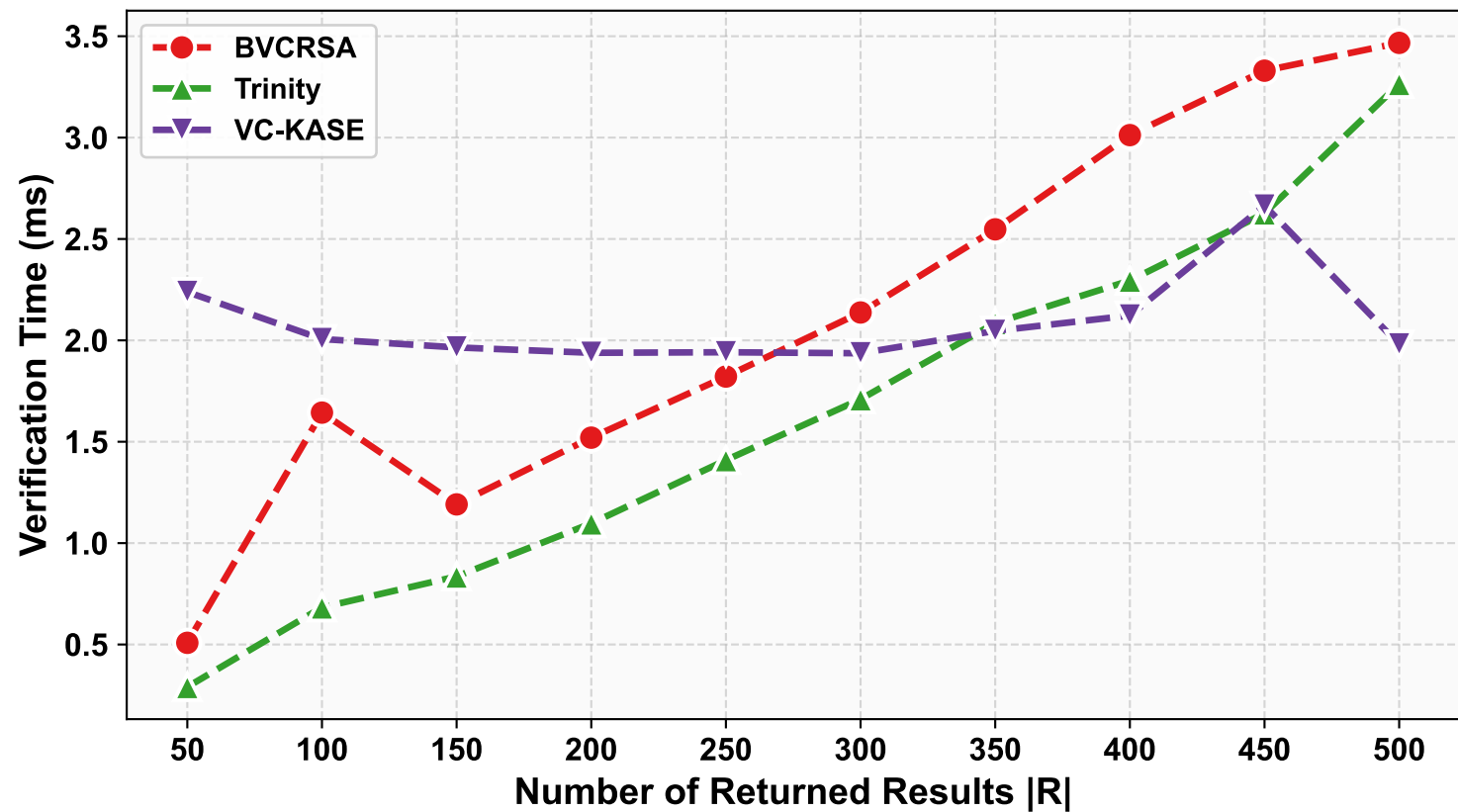
Verification Overhead vs Result Set Size
